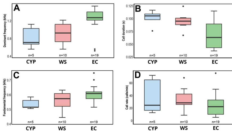
Fig. 9. Boxplot comparison of variation in the advertisement call traits between the Limnodynastes dorsalis group lineages redescribed herein, depicting variation in (A) dominant frequency (kHz), (B) call duration (s), (C) fundamental frequency (kHz), and (D) call rate (calls/min). Small dots represent outliers.
